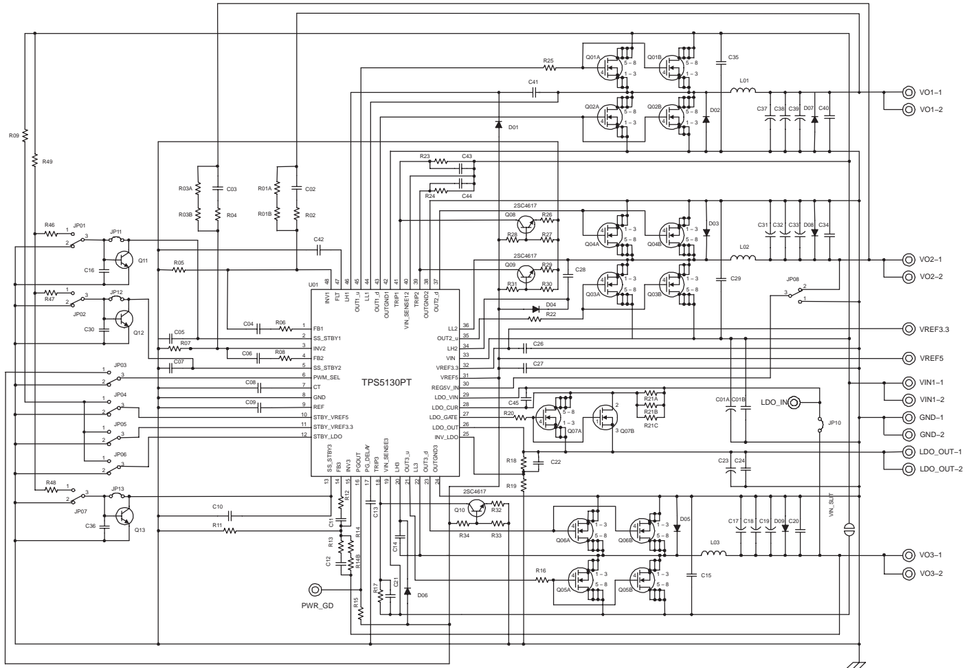
Figure 17. EVM Schematic
