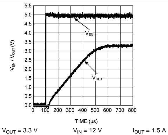
Figure 23. Startup – X Version (Resistive Load)
