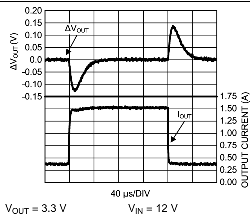
Figure 22. Load Transient – X Version
