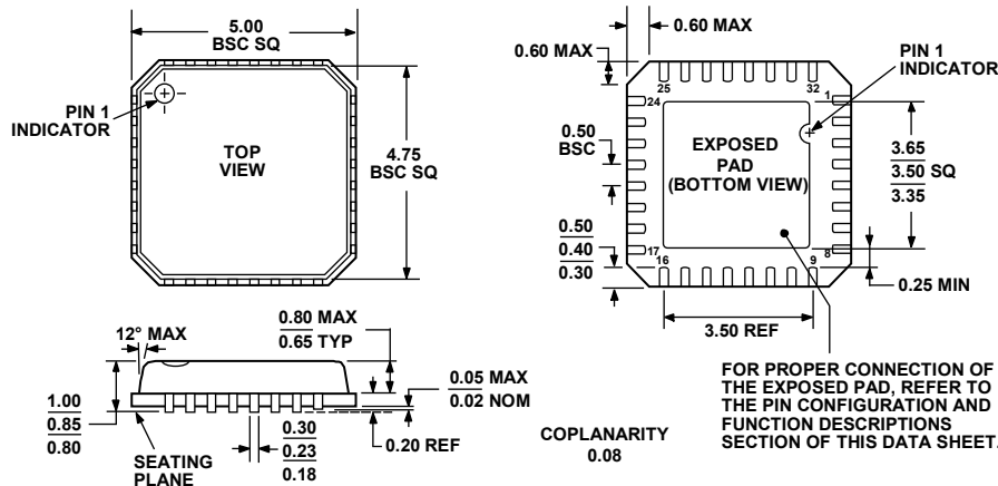
COMPLIANT TO JEDEC STANDARDS MO-220-VHHD-2 Figure 71. 32-Lead Lead Frame Chip Scale Package [LFCSP_VQ] 5 mm × 5 mm Body, Very Thin Quad (CP-32-4) Dimensions shown in millimeters
