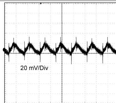
TIME (2 \mu\text{s/Div} ) 12 V_{IN} , 3.3 V_{OUT} at Full Load, BW = 250 MHz
