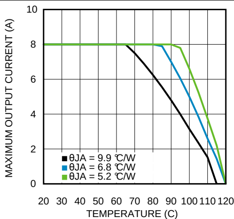
Figure 31. Thermal Derating
