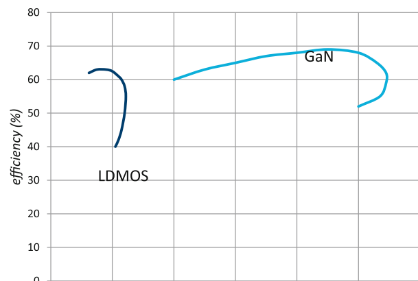
GaN vs LDMOS Comparison @ 2.1 GHz
