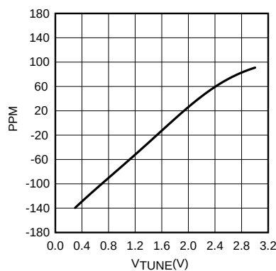
Figure 38. Example Tuning Curve, 20.48-MHz Crystal
