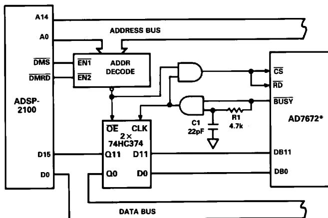
Figure 21. AD7672 - ADSP-2100 Interface
