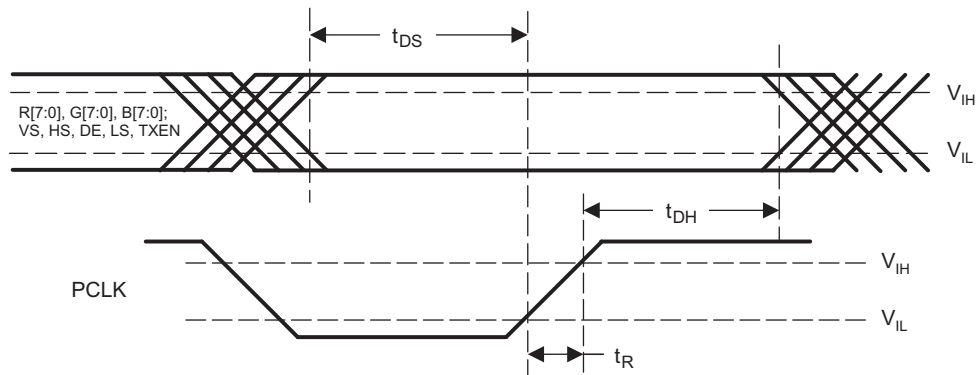
Figure 6. Setup/Hold Time
