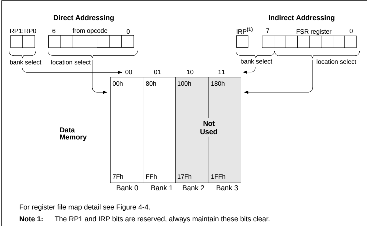
FIGURE 4-15: DIRECT/INDIRECT ADDRESSING
