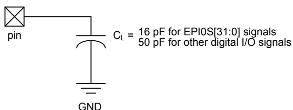
Figure 26-3. Load Conditions
