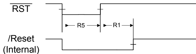
Figure 26-10. External Reset Timing ( \overline{\text{RST}} )
