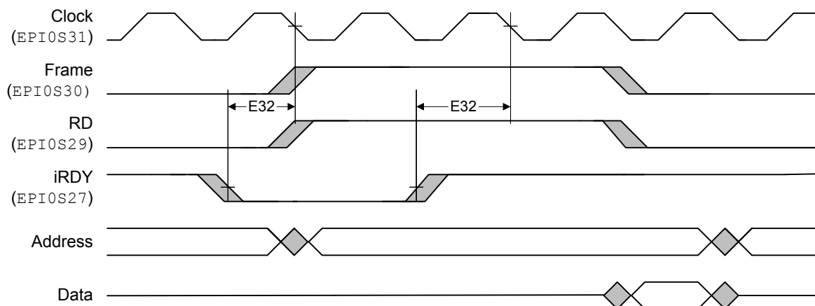
Figure 26-22. General-Purpose Mode iRDY Timing
