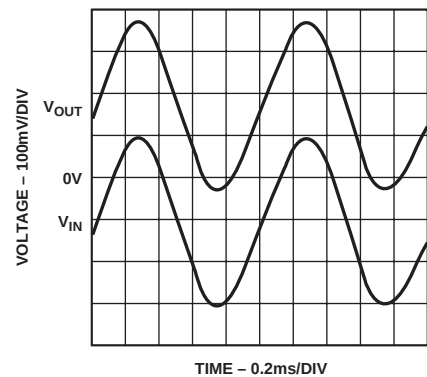
Figure 1. Input and Output Signals with V_{CM} < 0V
