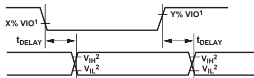
1 FOR V_{IO} \leq 3.0\text{ V} , X = 90 AND Y = 10 ; FOR V_{IO} > 3.0\text{ V} , X = 70 AND Y = 30 . 2 MINIMUM V_{IH}^2 AND MAXIMUM V_{IL}^2 USED. SEE THE DIGITAL INPUTS SPECIFICATIONS IN TABLE 3.
