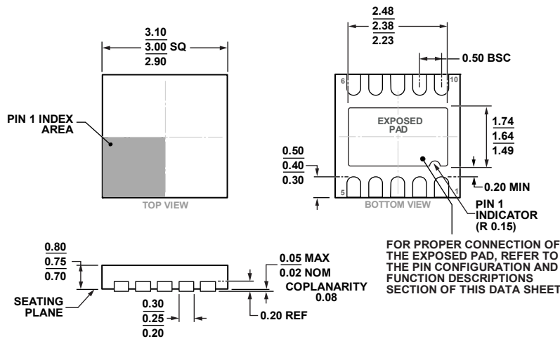
Figure 52. 10-Lead Lead Frame Chip Scale Package [LFCSP_WD] 3 mm × 3 mm Body, Very Very Thin, Dual Lead (CP-10-9) Dimensions shown in millimeters
