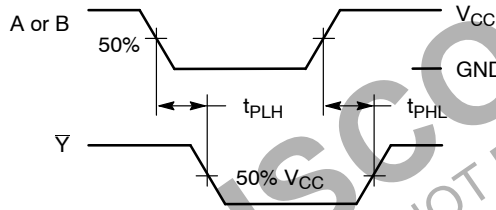
Figure 3. Switching Waveforms
