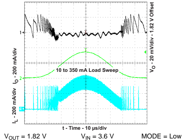
Figure 25. AC Load Transient Response, V_{OUT} = 1.82\text{ V} , V_{IN} = 3.6\text{ V}
