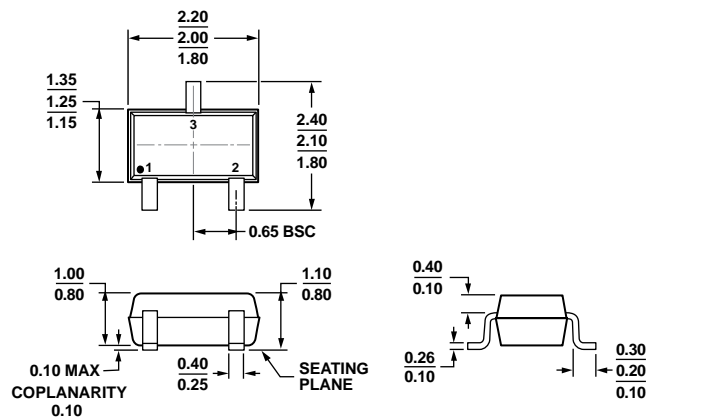
Figure 24. 3-Lead Thin Shrink Small Outline Transistor Package [SC70] (KS-3) Dimensions shown in millimeters
