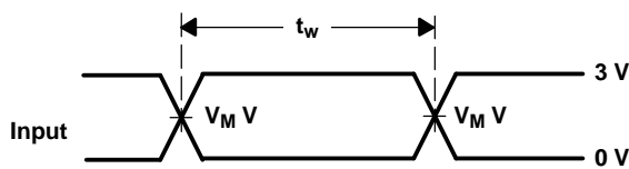
VOLTAGE WAVEFORMS PULSE DURATION ( V_M = 1.5\text{ V} for A port and V_{REF} for B port) (1)
