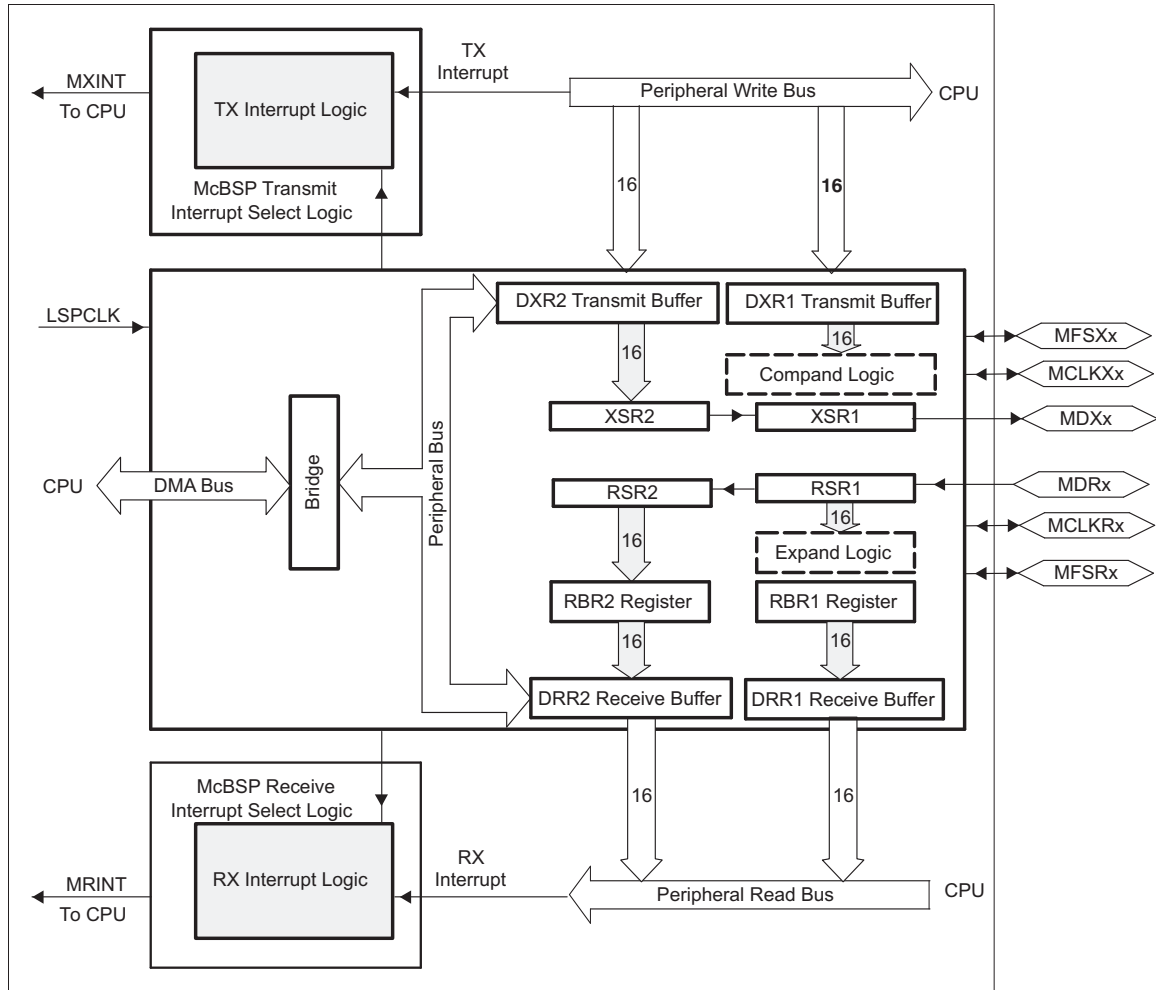
Figure 6-11. McBSP Module
