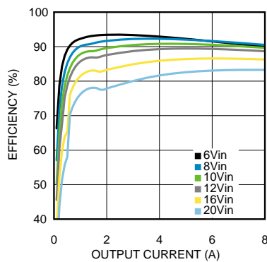
Figure 1. Efficiency 5-V Output at 25°C
