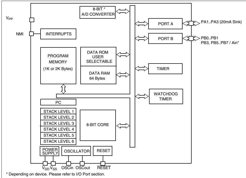
Figure 1. Block Diagram
