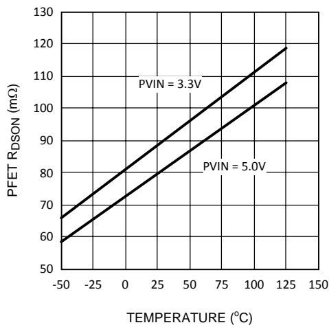
Figure 10. PMOS Switch R DSON vs Temperature
