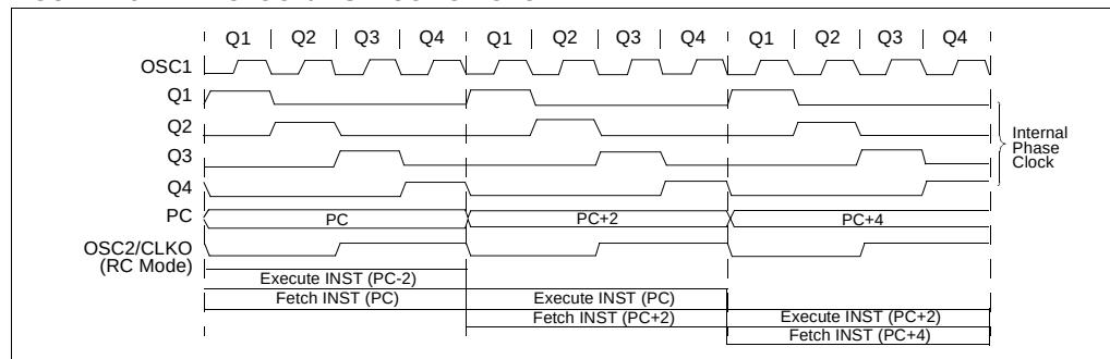
FIGURE 4-5: CLOCK/INSTRUCTION CYCLE
