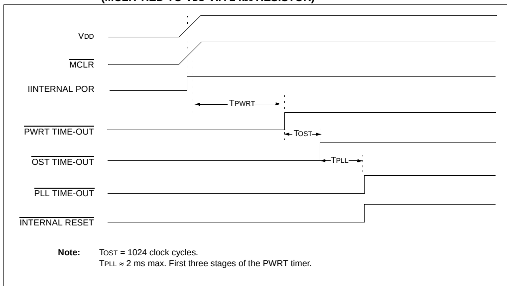
FIGURE 3-7: TIME-OUT SEQUENCE ON POR W/ PLL ENABLED (MCLR TIED TO V DD VIA 1 k \Omega RESISTOR)
