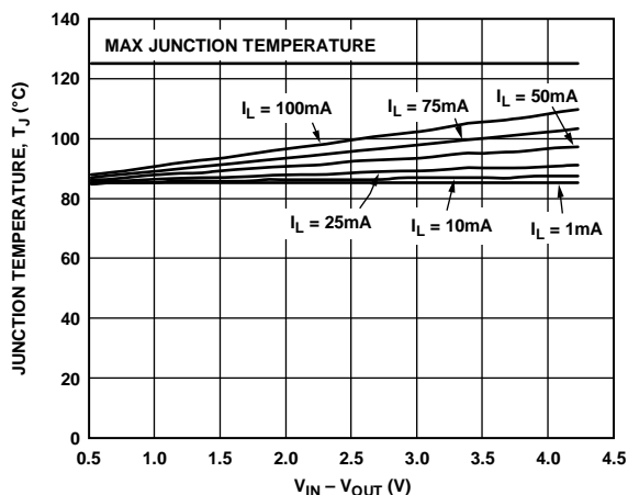
Figure 47. WLCSPP, T_B = 85^\circ\text{C}
