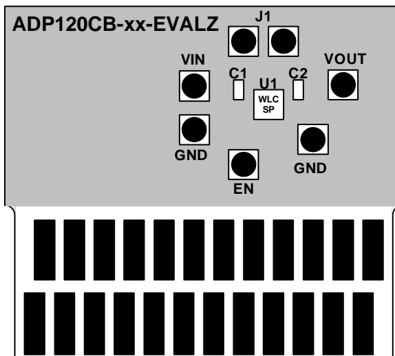
Figure 49. WLCSPP PCB Layout
