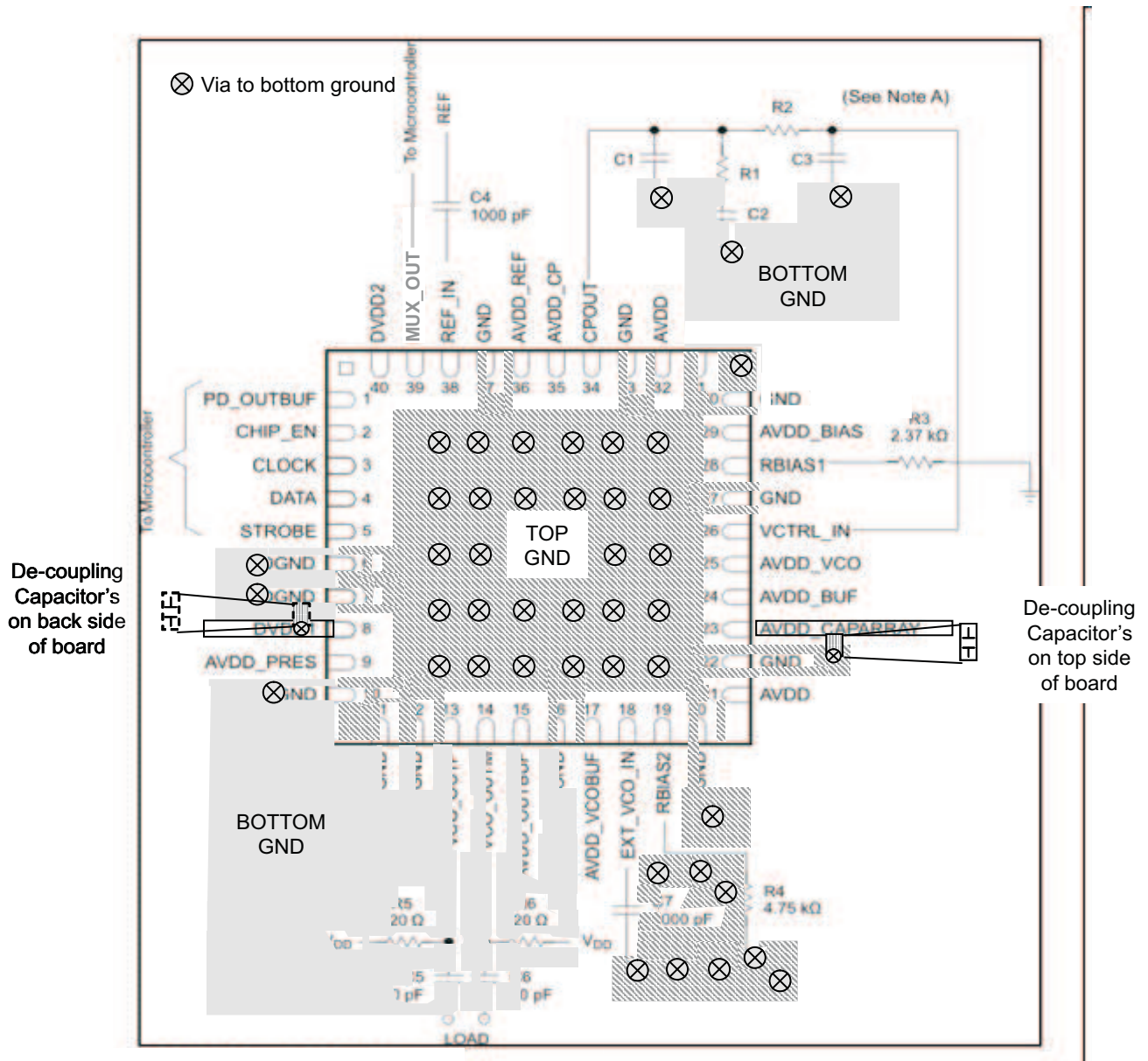
Figure 89. TRF3761 Layout
