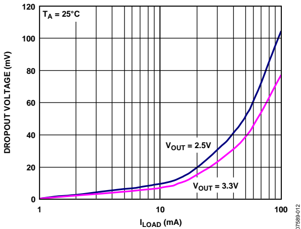
Figure 12. Dropout Voltage vs. Load Current, TSOT, V_{OUT} = 2.5\text{ V} and 3.3\text{ V}
