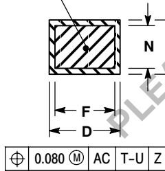
SECTION AE-AE
