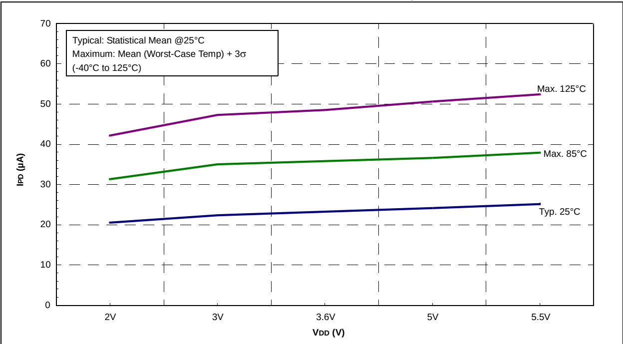
FIGURE 24-33: PIC16F722A/723A BOR IPD vs. VDD, VCAP = 0.1 \mu\text{F}
