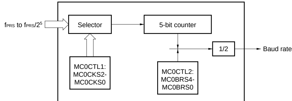
Figure 16-2. Block Diagram of Baud Rate Generator
