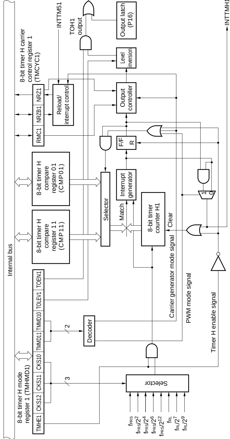
Figure 8-2. Block Diagram of 8-Bit Timer H1
