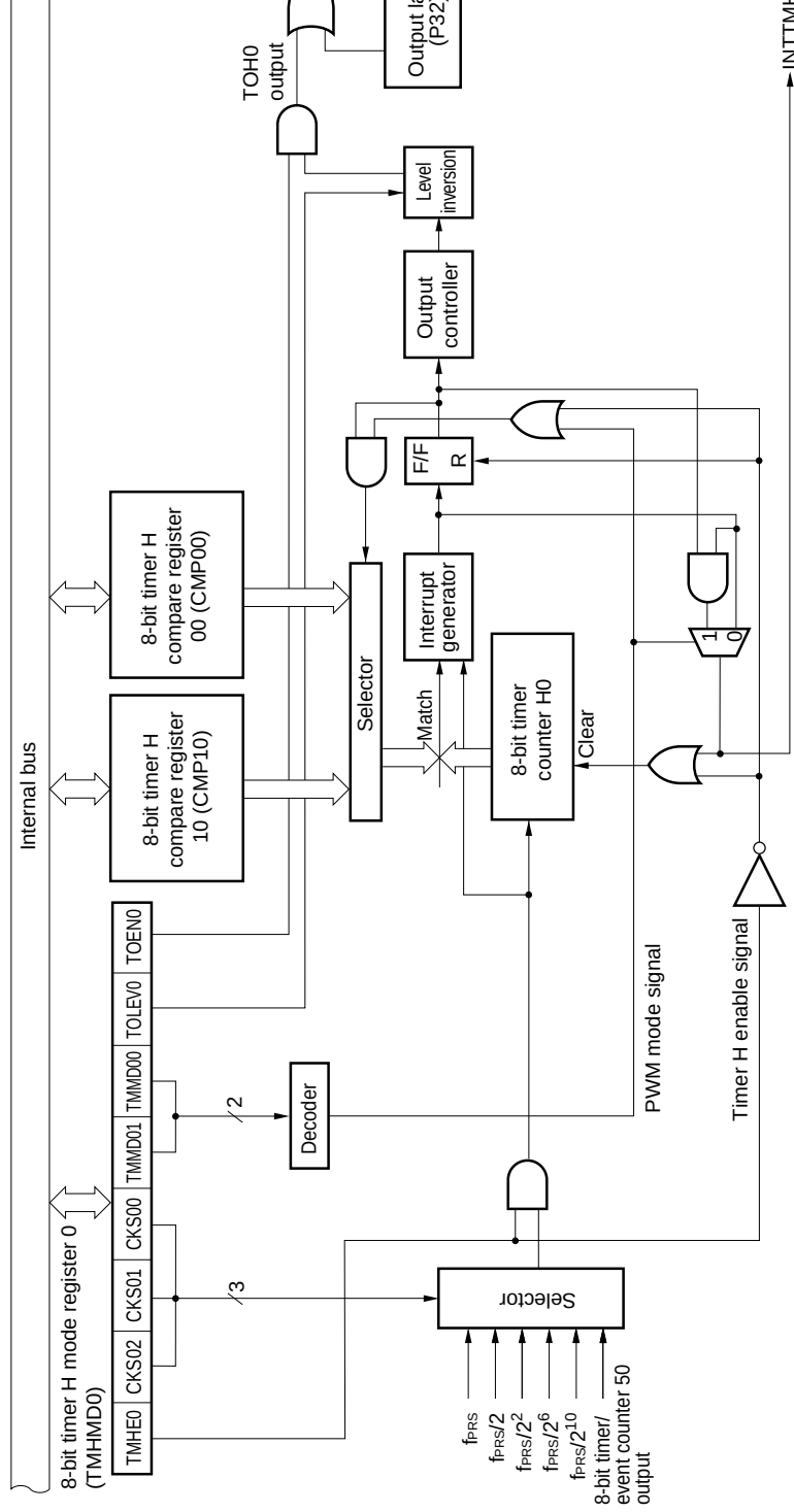
Figure 8-1. Block Diagram of 8-Bit Timer H0
