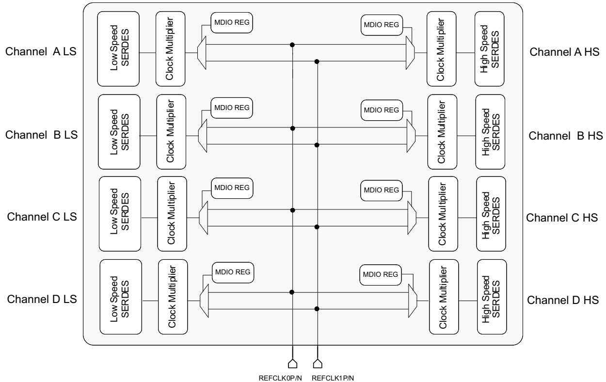
Figure 5-34. Reference Clock Architecture
