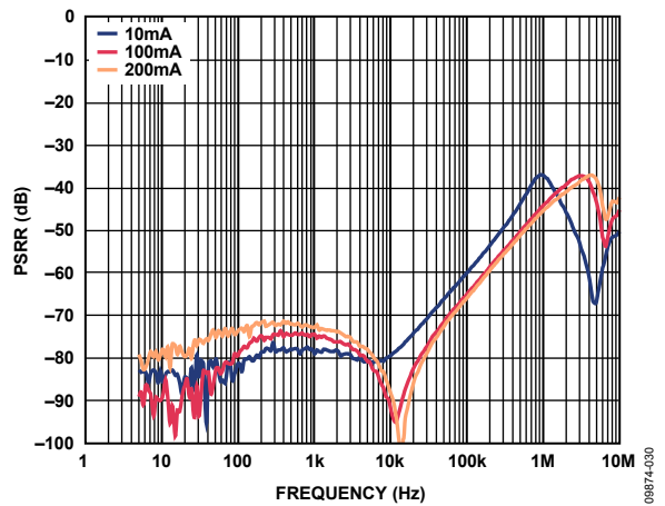
Figure 32. Power Supply Rejection Ratio vs. Frequency, V_{OUT} = 1.5 V , V_{IN} = 2.5 V , V_{RIPPLE} = 50 mV , C_{OUT} = 1 \mu F
