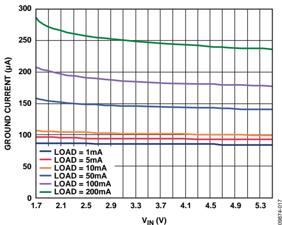
Figure 17. Ground Current vs. Input Voltage, All Outputs Loaded Equally, V_{RIPPLE} = 50\text{ mV} , C_{OUT} = 1\ \mu\text{F}
