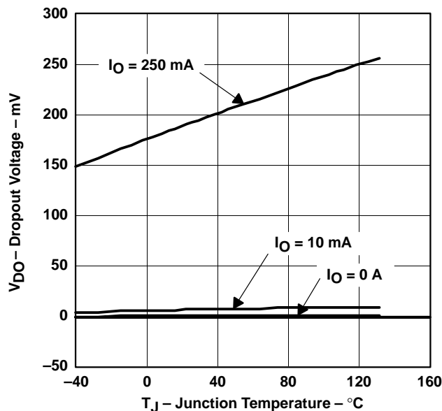
TPS77333 DROPOUT VOLTAGE VS JUNCTION TEMPERATURE
