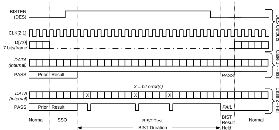
Figure 31. BIST Waveforms
