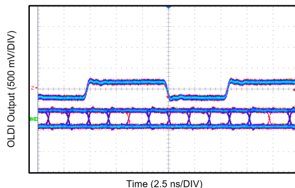
Figure 54. OpenLDI Clock and Data Output at 74.25-MHz Pixel Clock
