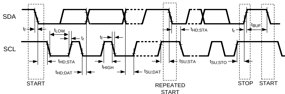
Figure 14. Serial Control Bus Timing Diagram
