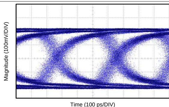
Figure 53. Loop-Through CML Output at 2.6-Gbps Serial Line Rate
