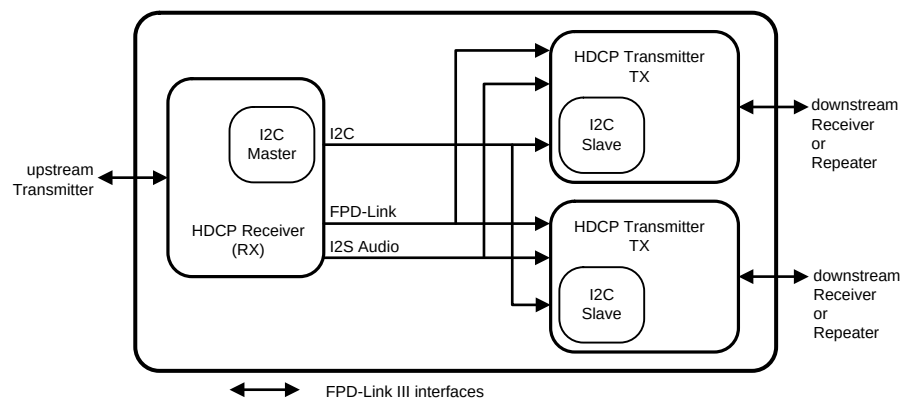
Figure 27. HDCP 1:2 Repeater Configuration
