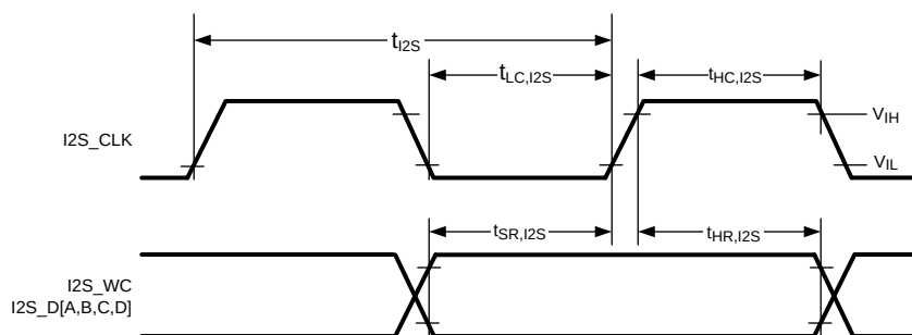
Figure 15. I2S Timing
