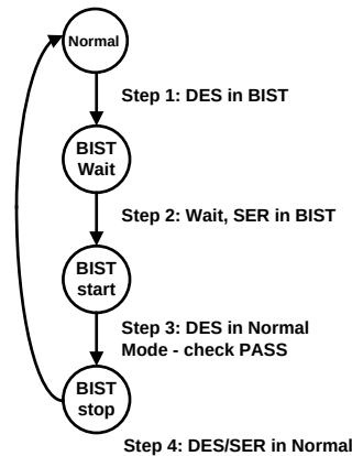
Figure 30. BIST Mode Flow Diagram
