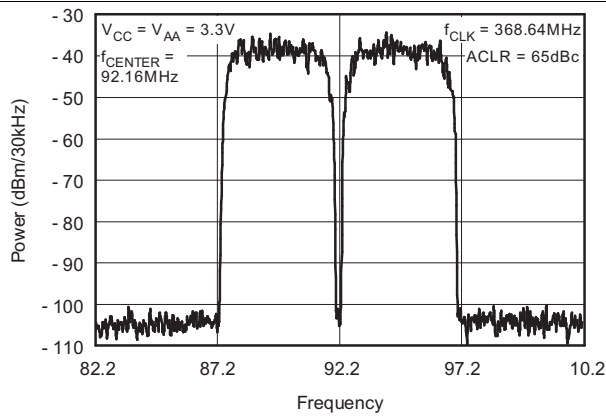
Figure 11. W-CDMA TM1 Dual Carrier Power vs Frequency
