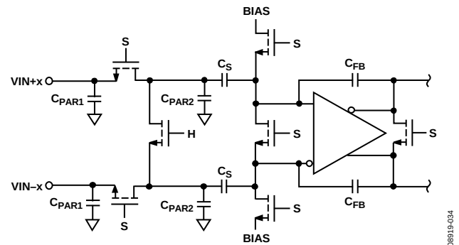
Figure 77. Switched-Capacitor Input
