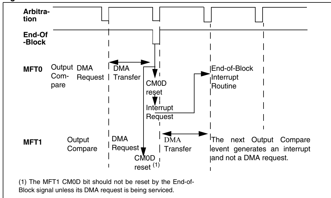
Figure 208. Multifunction timer
