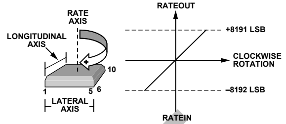
Figure 4. RATEOUT Level Increase with Clockwise Rotation Increase
