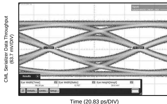
DS80PCI810 Settings: EQA = Level 4, VODA = Level 6 TJ (1.0E-12) = 33.0 ps Figure 20. TL1 = 15 Inch 5-Mil FR4 Trace, TL2 = 10 Inch 5-Mil FR4 Trace, DS80PCI810 CHA_0, 8 Gbps
