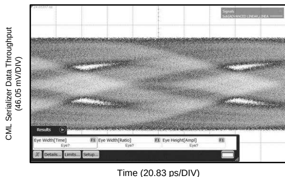
No Repeater Used TJ (1.0E-12) = Not Available Due to Closed Eye Figure 19. TL1 = 15 Inch 5-Mil FR4 Trace, TL2 = 10 Inch 5-Mil FR4 Trace, No Repeater, 8 Gbps
