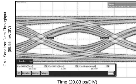
DS80PCI810 Settings: EQA = Level 4, VODA = Level 6 TJ (1.0E-12) = 41.4 ps Figure 18. TL = 5-Meter 30-AWG 100 \Omega Twin-Axial Cable, DS80PCI810 CHA_0, 8 Gbps
