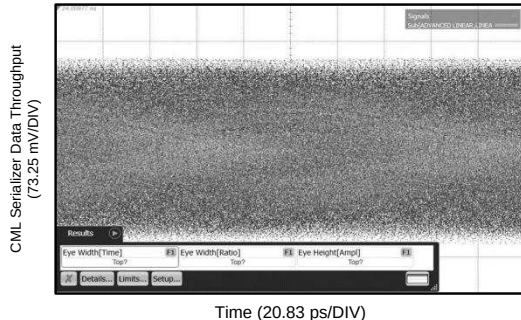
No Repeater TJ (1.0E-12) = Not Available Due to Closed Eye Figure 17. TL = 5-Meter 30-AWG 100 \Omega Twin-Axial Cable, No Repeater, 8 Gbps
