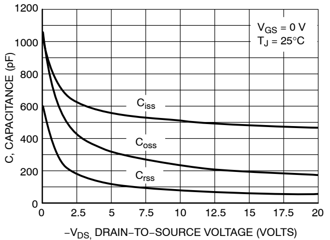
Figure 6. Capacitance Variation
