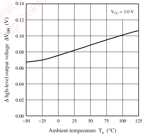
Δ high-level output voltage — Ambient temperature
