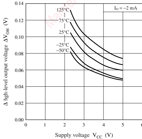
Δ high-level output voltage — Supply voltage
