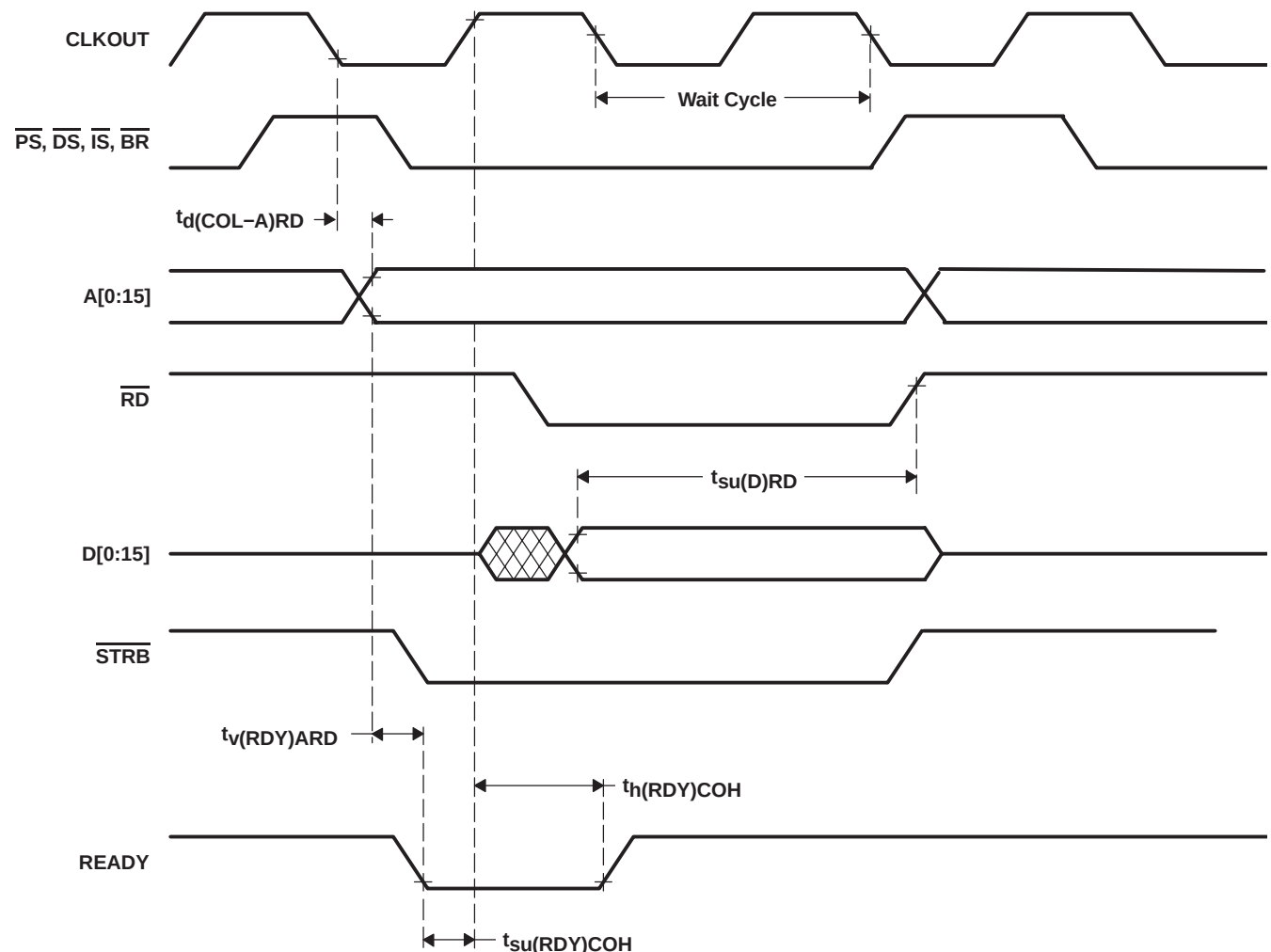
Figure 39. Ready-on-Read Timings
