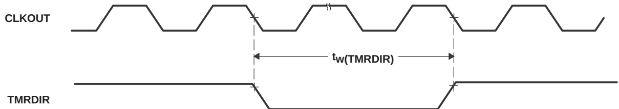
Figure 28. Capture/TMRDIR Timing
