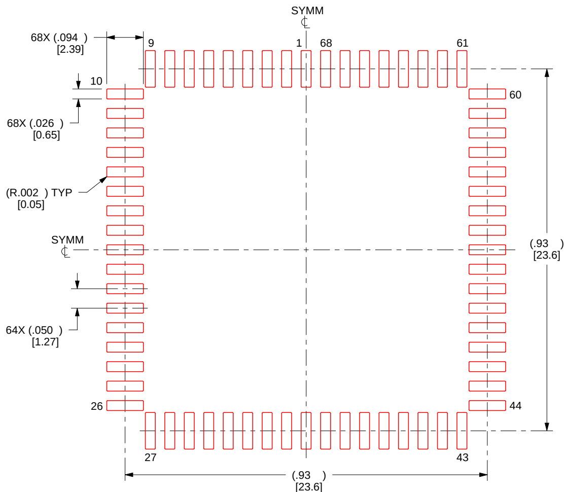
SOLDER PASTE EXAMPLE SCALE:4X
