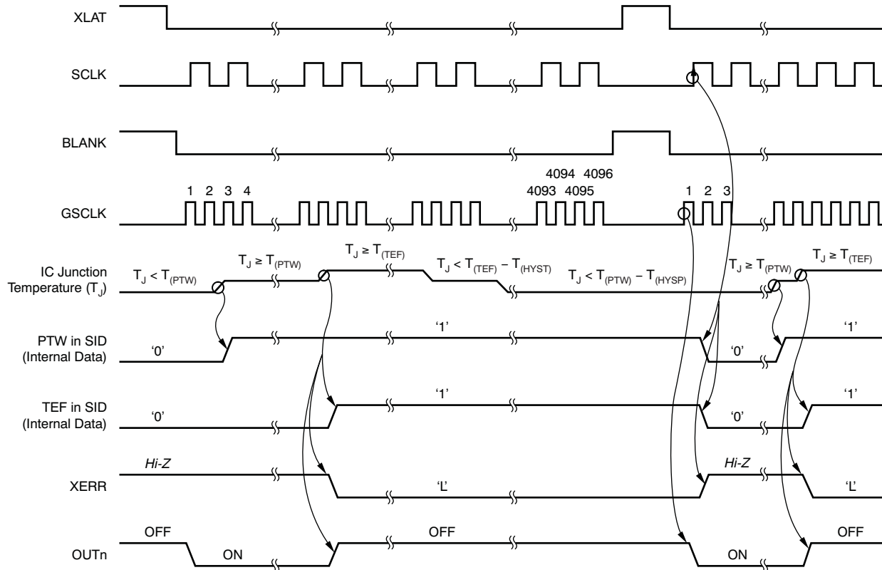
Figure 32. TEF/TSD/XERR Timing
