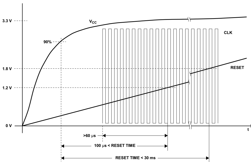
Figure 4-1. Reset Timing
