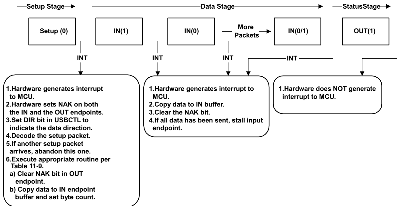
Figure 5-13. Control Read Transfer
