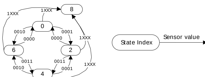
Figure 21.14. FSM example 2
