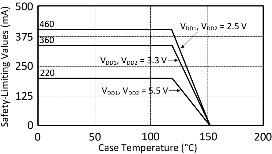
Figure 14. (WB SOIC-16) Thermal Derating Curve for Safety Limiting Current
