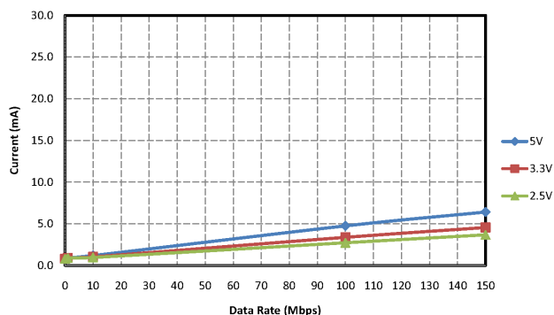
Figure 6. Si8610 Typical V_{DD2} Supply Current vs. Data Rate 5, 3.3, and 2.5V Operation (15 pF Load)
