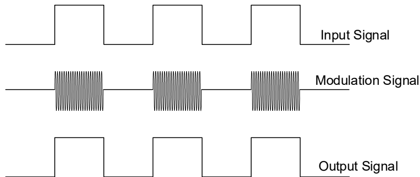
Figure 2. Modulation Scheme
