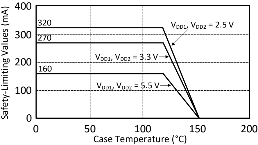
Figure 15. (SOIC-8) Thermal Derating Curve for Safety Limiting Current
