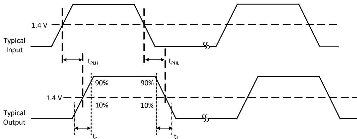
Figure 12. Propagation Delay Timing
