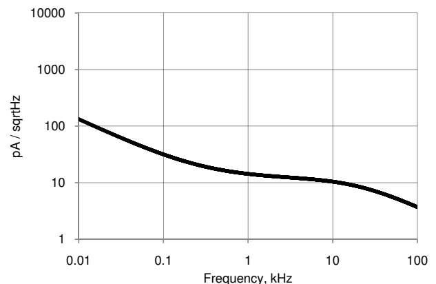
Figure 11-60. IDAC Current Noise, 255 \mu A Mode, Source Mode, Fast Mode, V_{DDA} = 5 V
