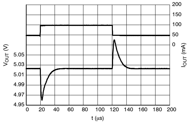
Figure 28. Load Transients, 8.0 V Version, I_{OUT} = 1 - 20 \text{ mA} , t_R = t_F = 50 \mu\text{s} , V_{IN} = 11.0 \text{ V}
