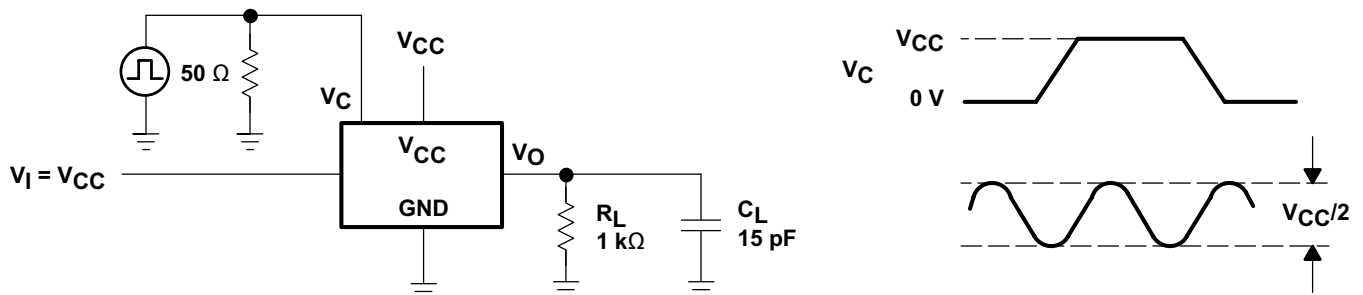
Figure 6. Switching Time (t PZL , t PLZ , t PZH , t PHZ ), Control to Signal Output
