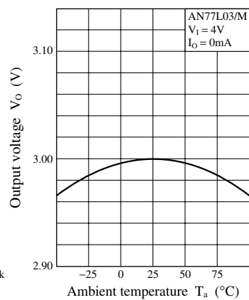
Output voltage temperature characteristic V_O — T_a
