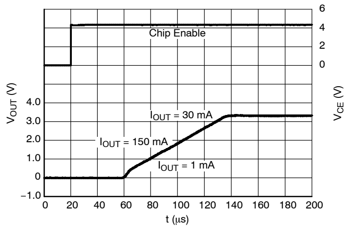
Figure 35. Start-up, 3.3 V Version, V IN = 4.3 V
