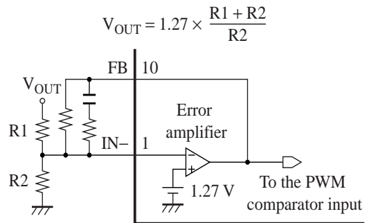
Figure 2. Connection method of error amplifier
