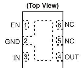
U-DFN2020-6 (Fixed Output) (SN Package)
